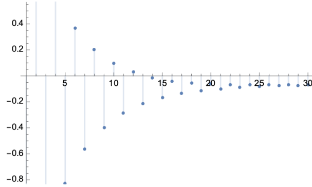
FIGURE 2. u_{1/2,-3/2}(n) for n \in [1, 30] \cap \mathbb{N} .
