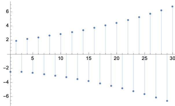
FIGURE 3. u_{1/2,-7/5}(n) for n \in [1, 30] \cap \mathbb{N} .
