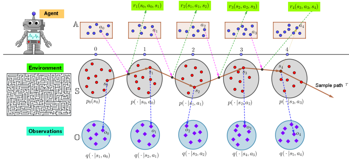
Figure 4: Reinforcement Learning
