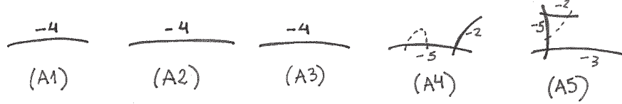
Figure 1: Options for \kappa = 1
